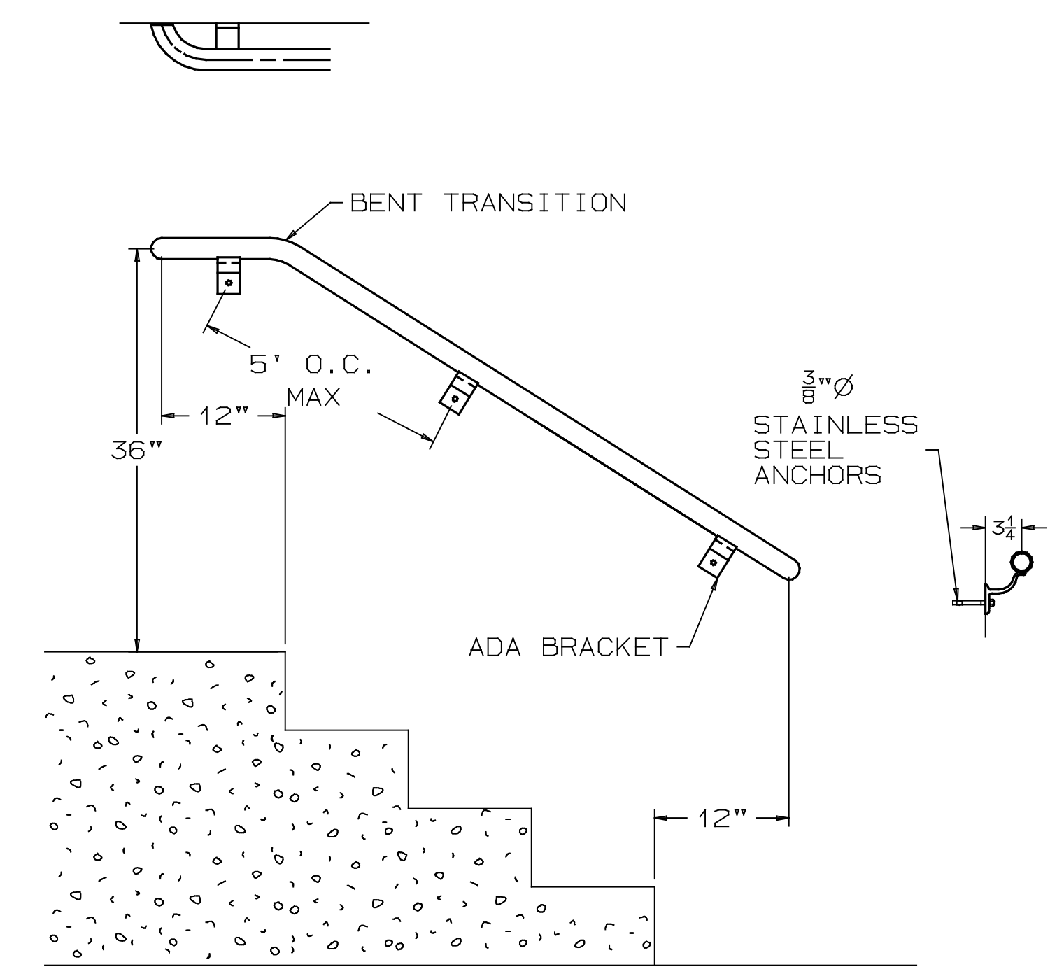
TYPICAL WALL MOUNTED HANDRAIL
