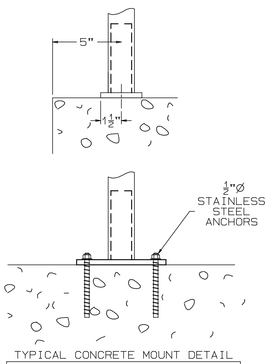
TYPICAL GUARDRAIL
