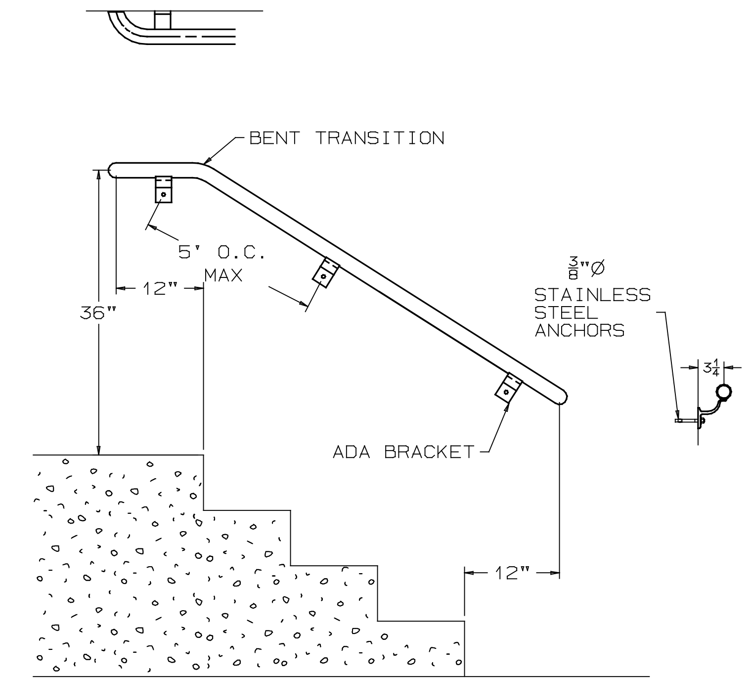
TYPICAL WALL MOUNTED HANDRAIL
