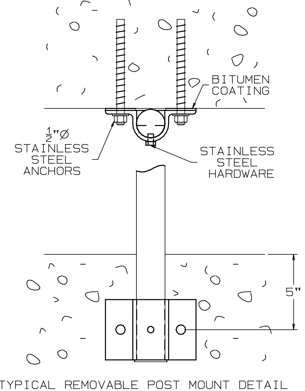
TYPICAL REMOVABLE POST MOUNT DETAIL
