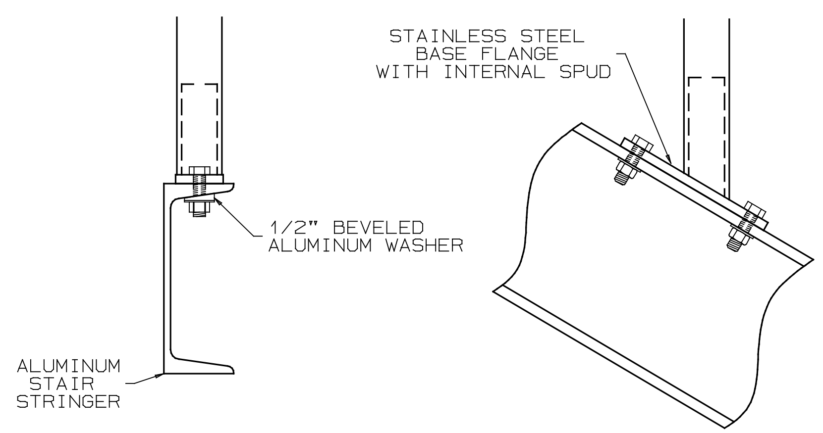
TYPICAL POST TO STRINGER MOUNT DETAIL
