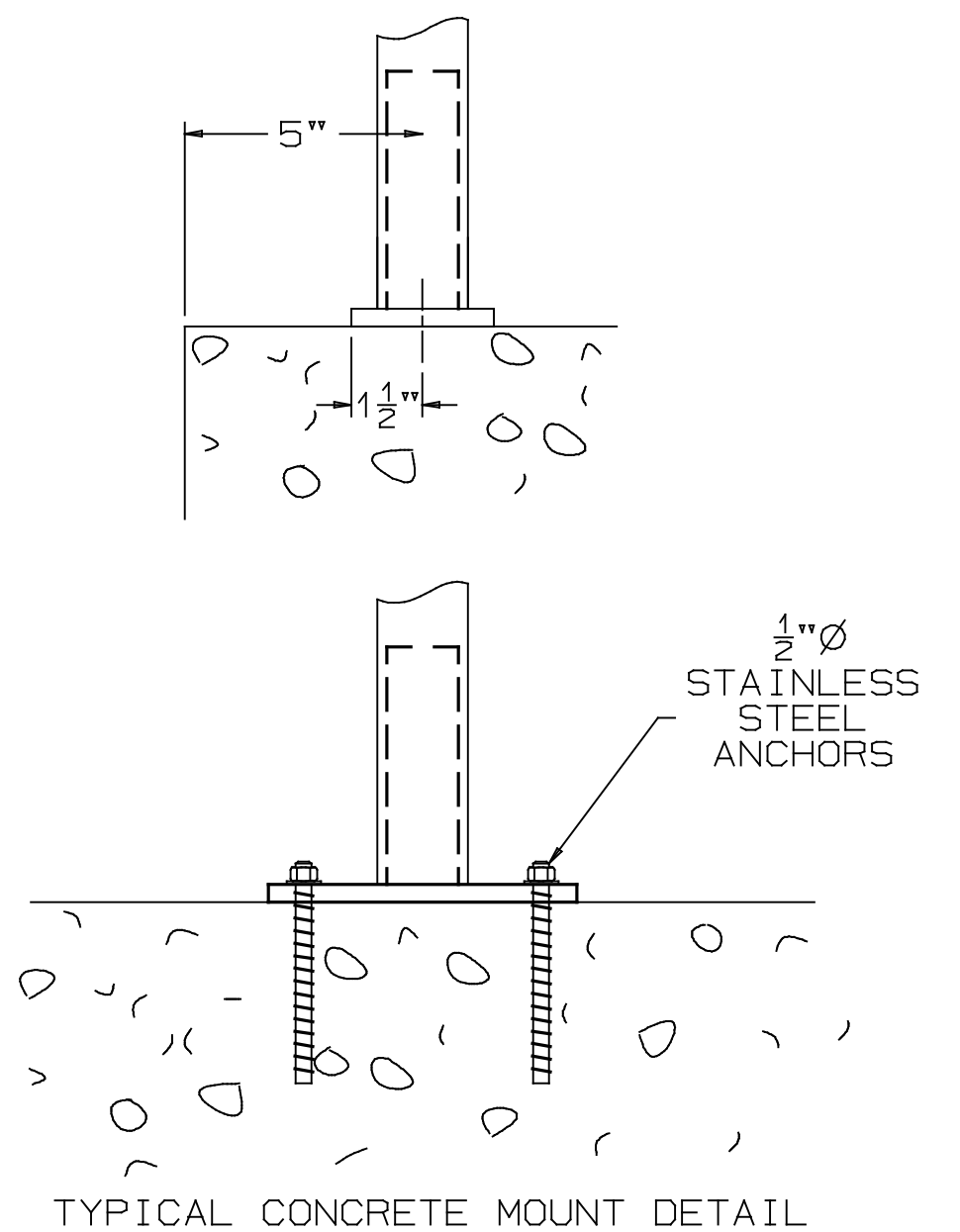
TYPICAL CONCRETE MOUNT DETAIL
