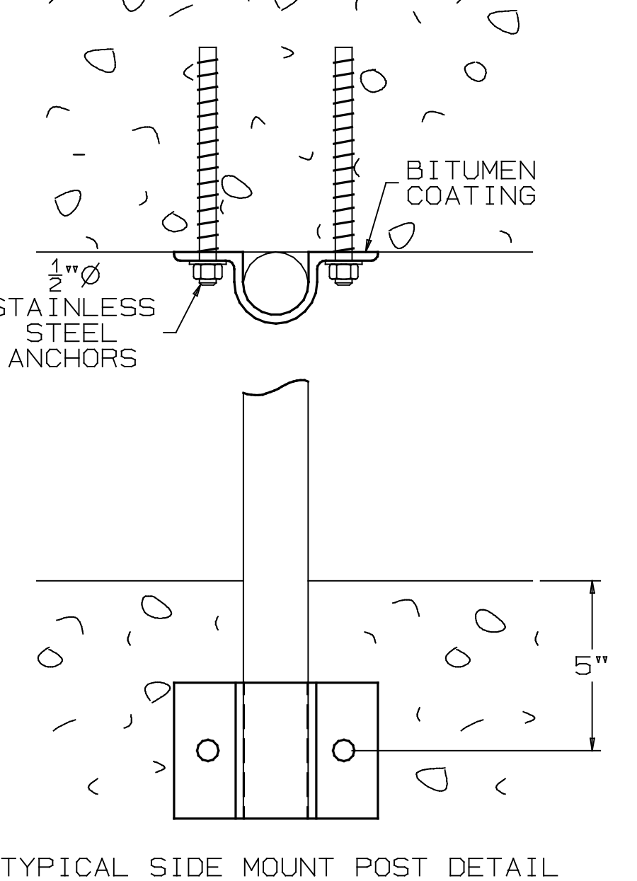
TYPICAL SIDE MOUNT POST DETAIL
