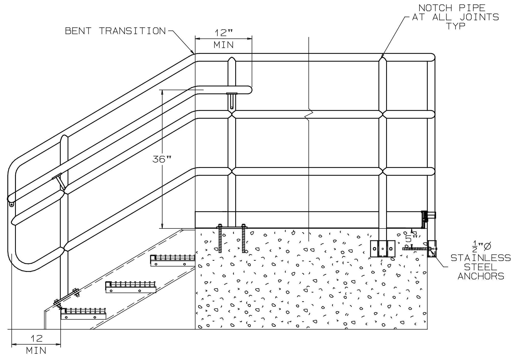
TYPICAL GUARDRAIL AT METAL STAIR
