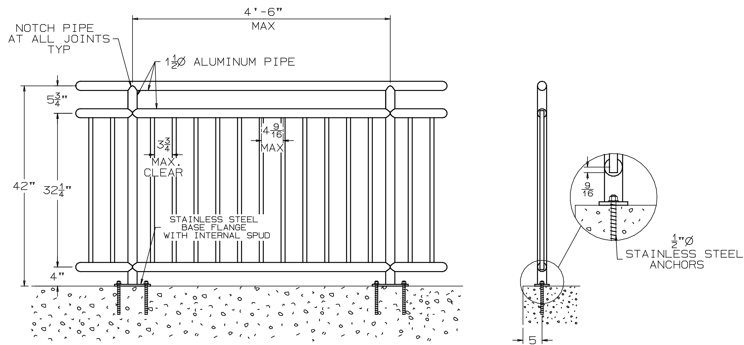
TYPICAL GUARDRAIL
