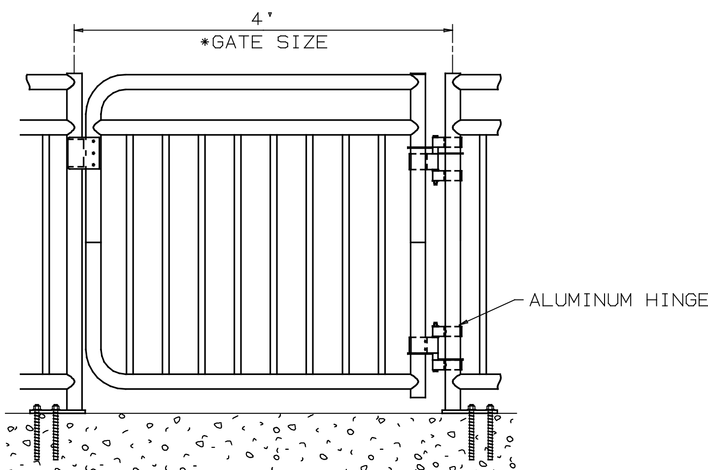
TYPICAL ALUMINUM SWING GATE
