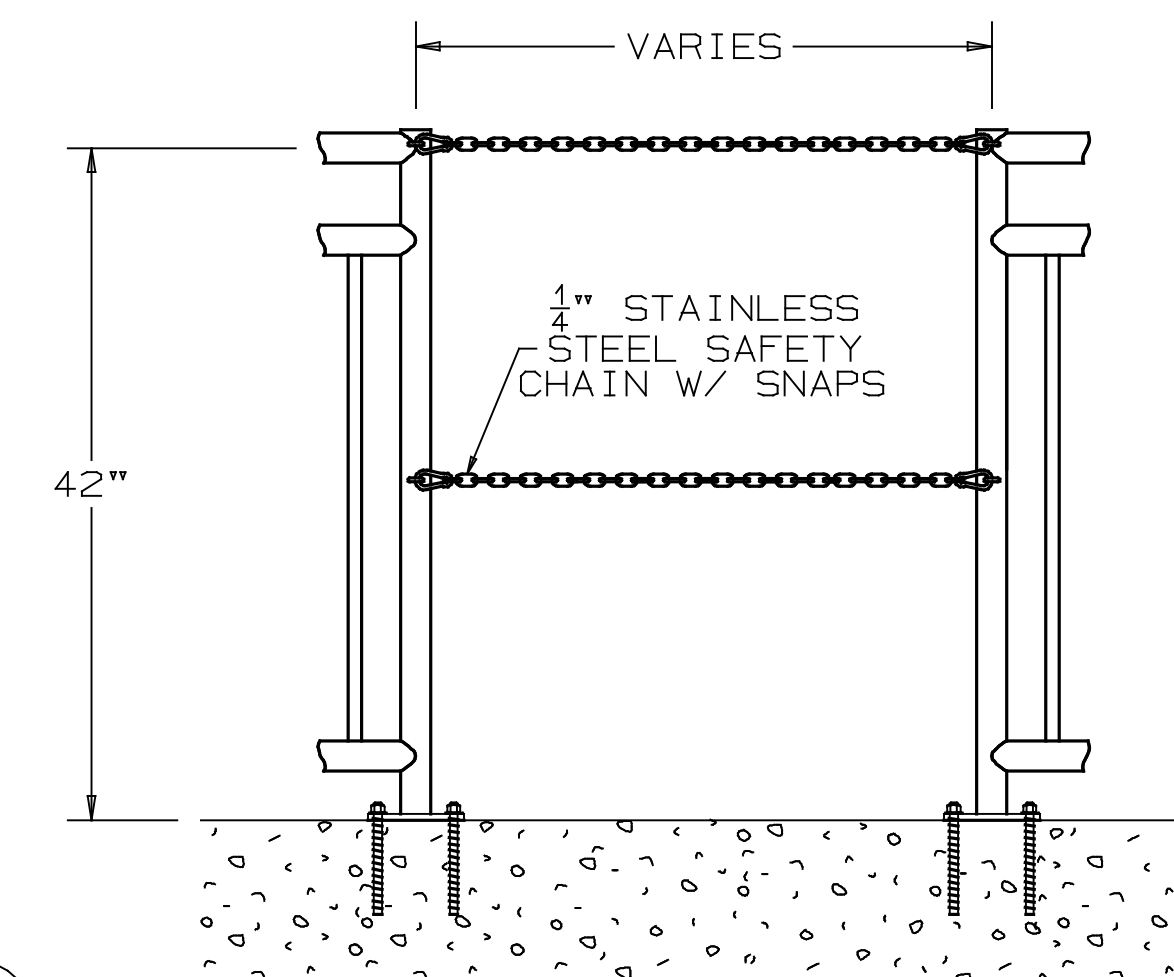
TYPICAL RAIL OPENING W/ SAFETY CHAIN
