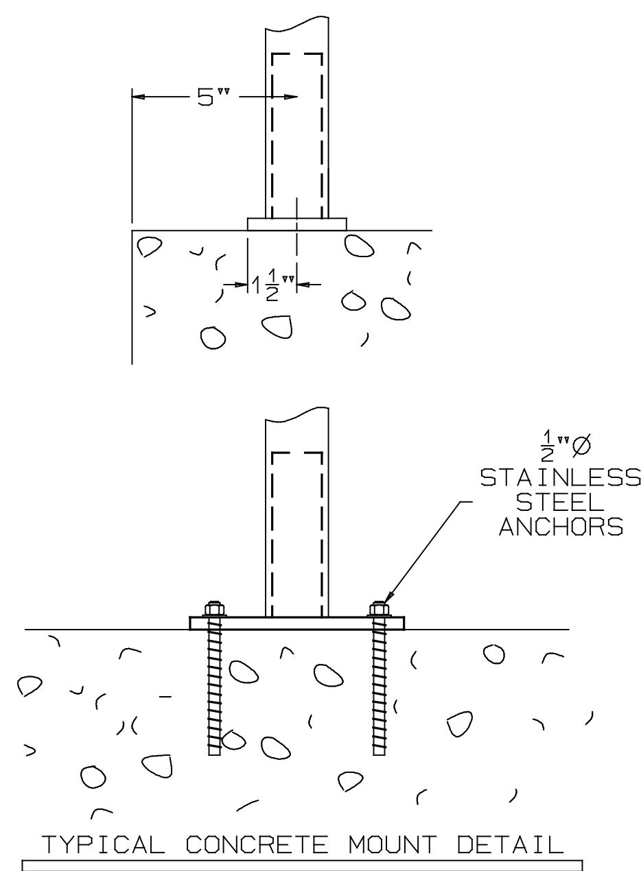
TYPICAL GUARDRAIL
